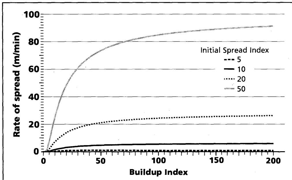
Figure 20. Rate of spread for the Mature Jack or Lodgepole Pine (C-3) fuel type for selected Initial Spread Index (ISI) and Buildup Index (BUI) values.
