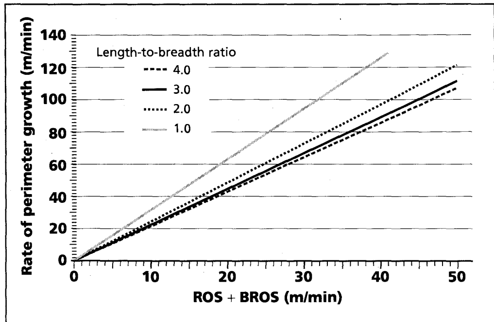
Figure 51. Perimeter growth rate values for selected head fire rates of spread (ROS), back fire rates of spread (BROS), and length-to-breadth ratios.
