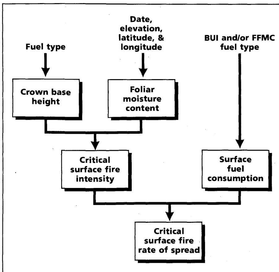
Figure 34. Inputs and process used to predict the critical surface fire rate of spread.
