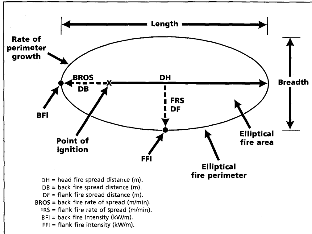
Figure 39. Conceptual diagram illustrating the secondary outputs produced by the FBP System.
