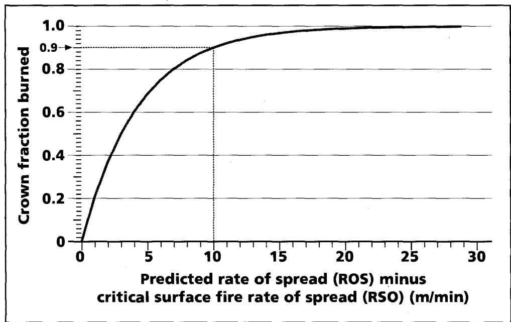
Figure 35. Crown fraction burned curve.
