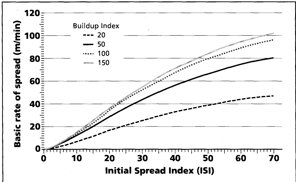
Figure 21. Rate of spread for the Boreal Spruce (C-2) fuel type for selected Initial Spread Index (ISI) and Buildup Index (BUI) values.
