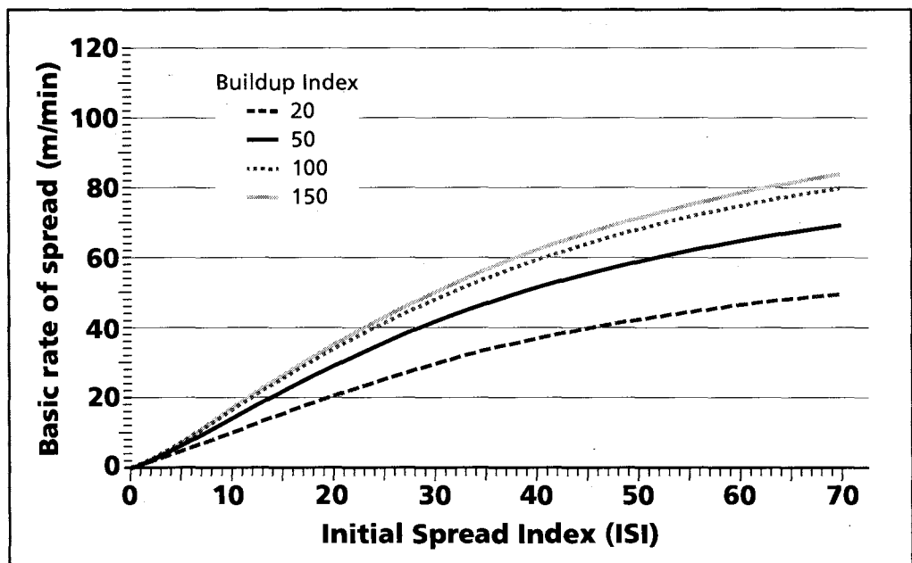
Figure 22. Rate of spread for the Jack or Lodgepole Pine (S-1) fuel type for selected Initial Spread Index (ISI) and Buildup Index (BUI) values.
